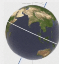
CHANGES IN OBLIQUITY (TILT) IN A 41,000-YEAR CYCLE
