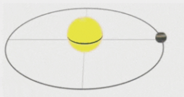
CHANGES IN ECCENTRICITY (ORBIT SHAPE) IN A 100,000-YEAR CYCLE
