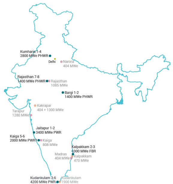
Planned Nuclear Power Plants in India
