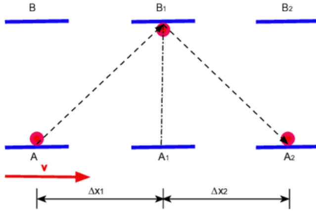
Clock moving at a constant velocity v respect to an observer at rest
